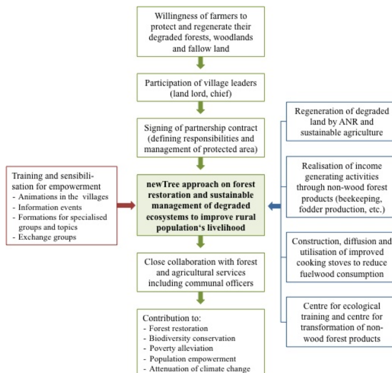
Figure 2: NewTree approach.
