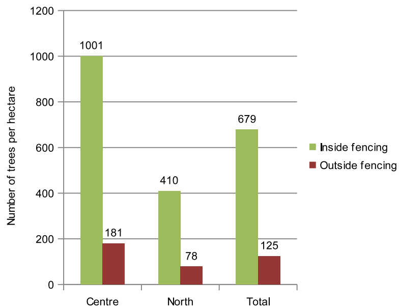
Figure 5: Average number ( A_n ) of species and trees per hectare inside and outside of the protected area.
