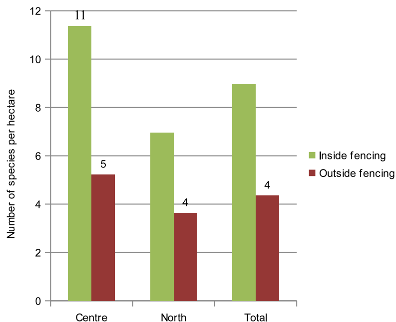
Figure 4: Tree species diversity both central and northern regions.
