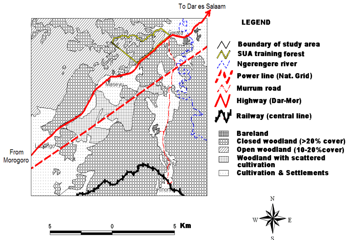
Figure 2: Land cover map for the study area in July 1975
